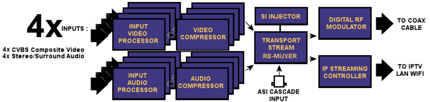
BLOCK DIAGRAM
